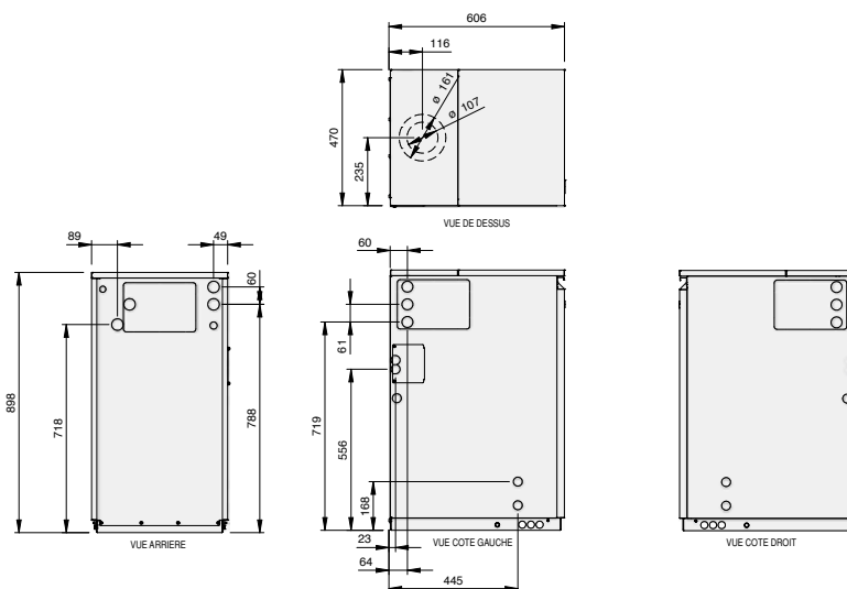
Dimensions chaudières Vortex Utility Bas NOx 32 kW
